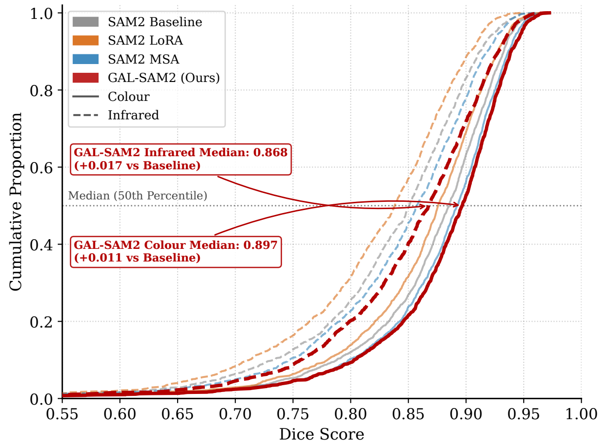
A. Cumulative Distribution of Dice Score (YOLO Automated Mode)
