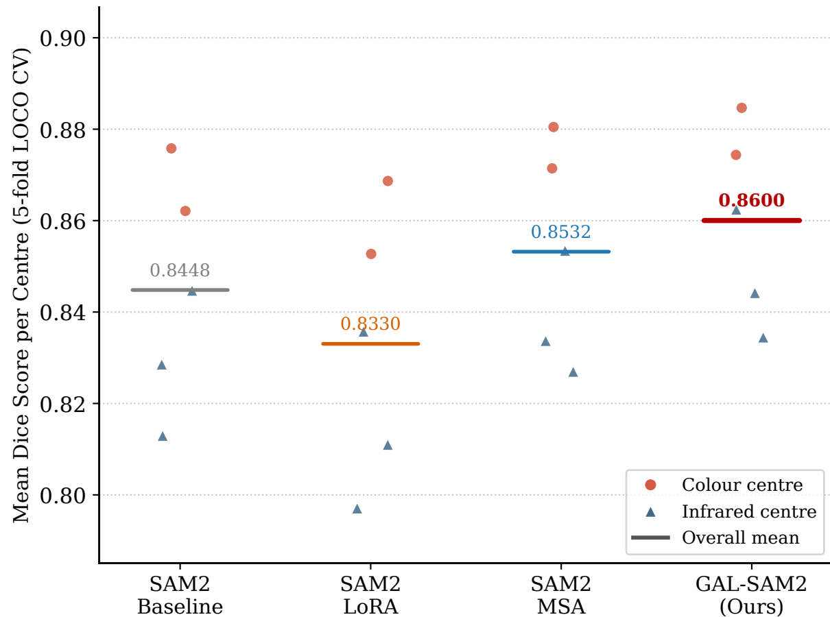
B. Per-Centre Dice Consistency (Each dot = one held-out centre; bar = overall mean)
