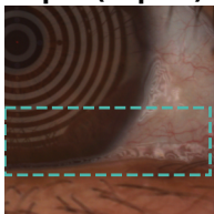
Input (Expert)
