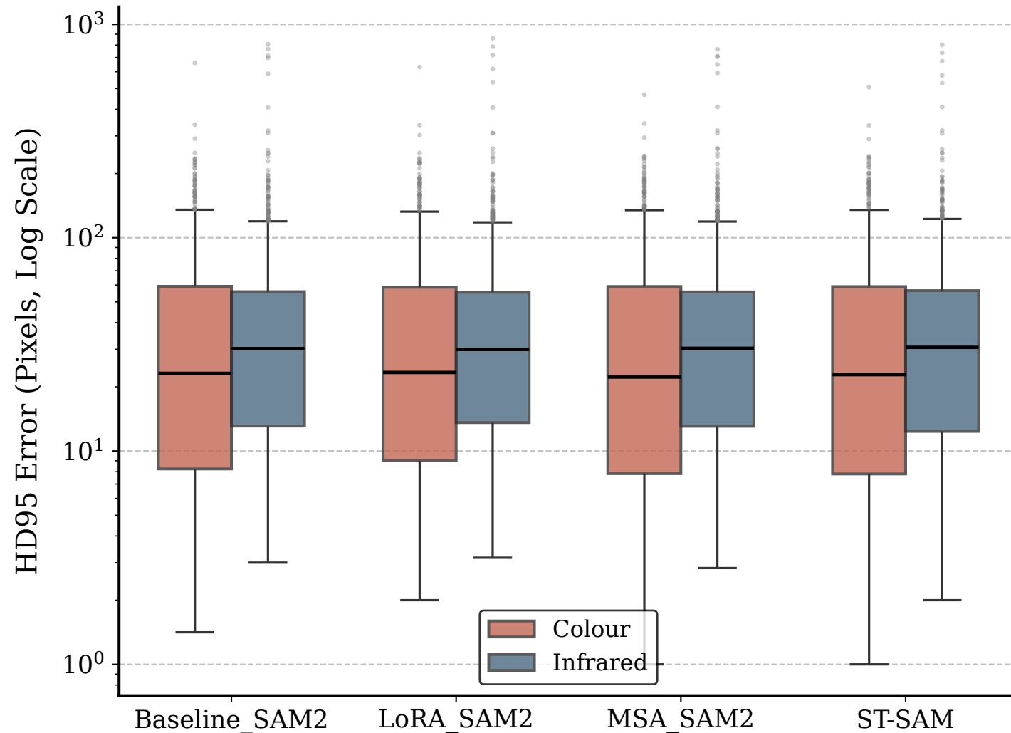
Boundary Drift under Automated YOLO Prompts
