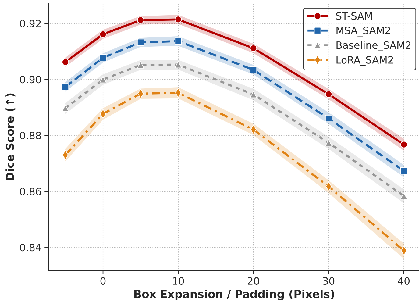
Dice vs. Box Expansion (Tolerance to Jittering Noise)
