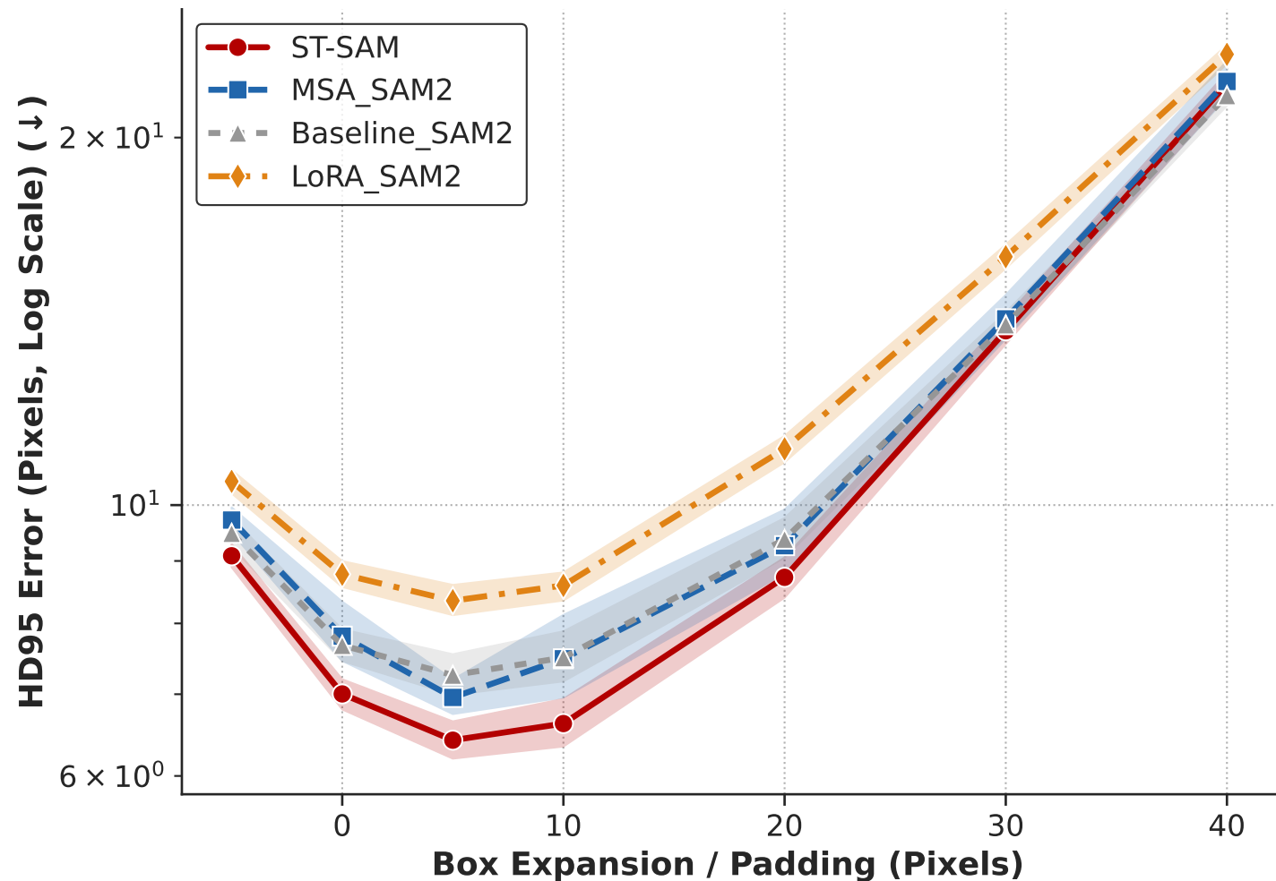
HD95 vs. Box Expansion (Boundary Drift Robustness)
