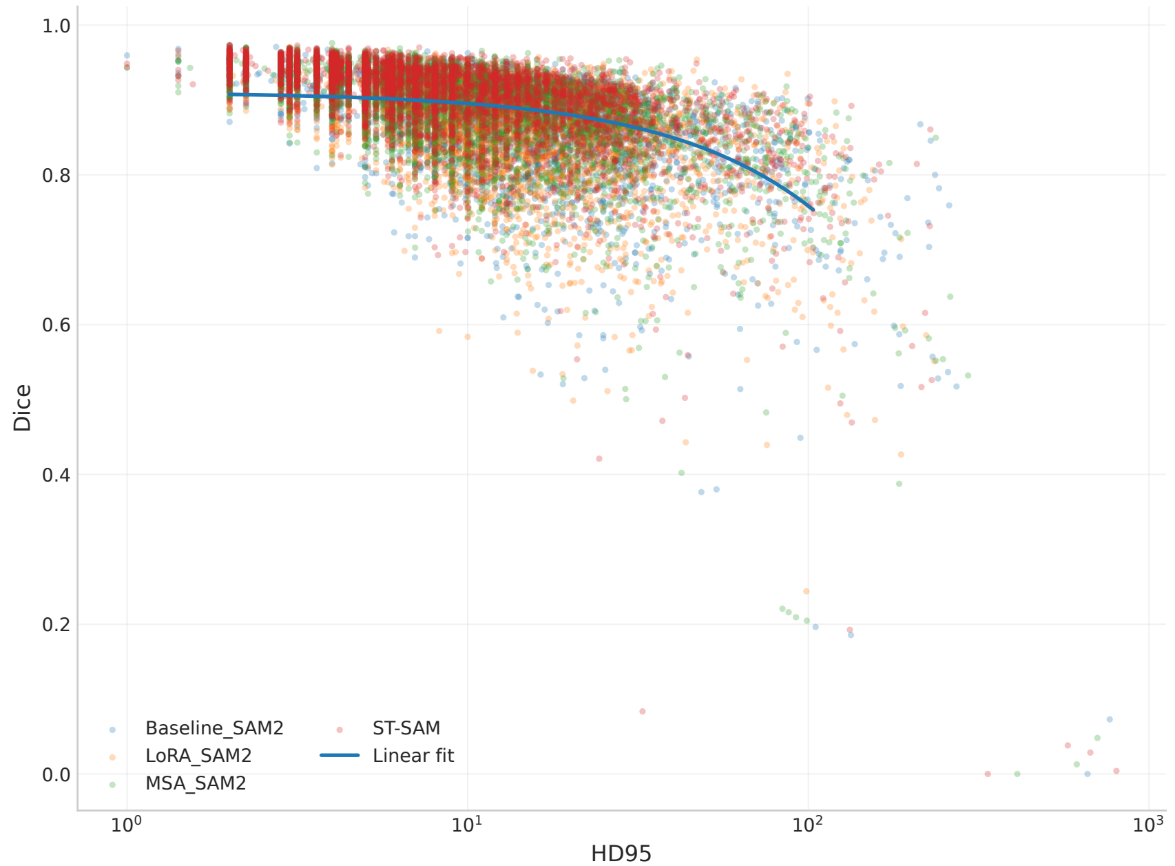
Dice vs HD95 Scatter
