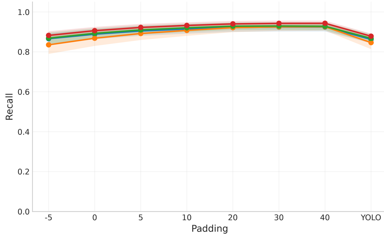
Recall vs Padding (fold mean \pm 95% CI)
