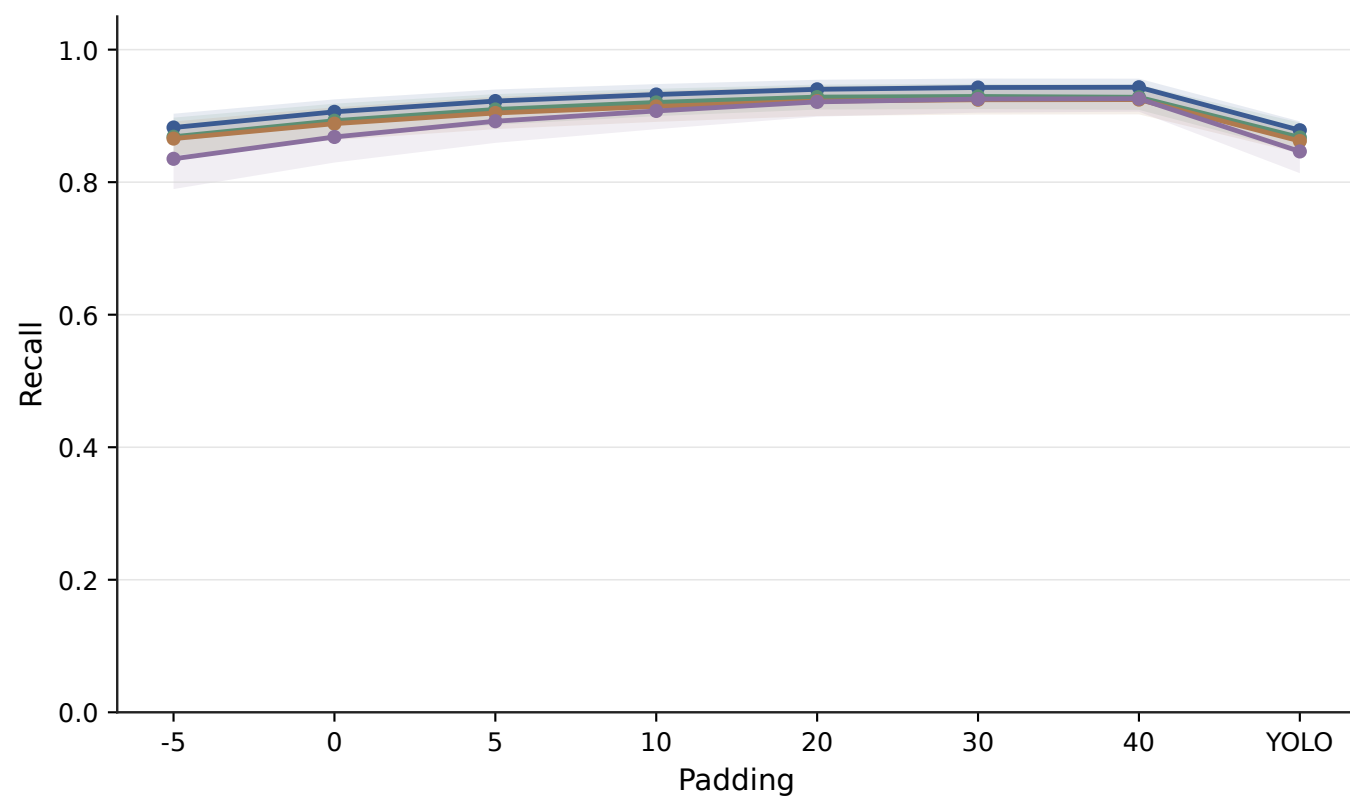
Recall
