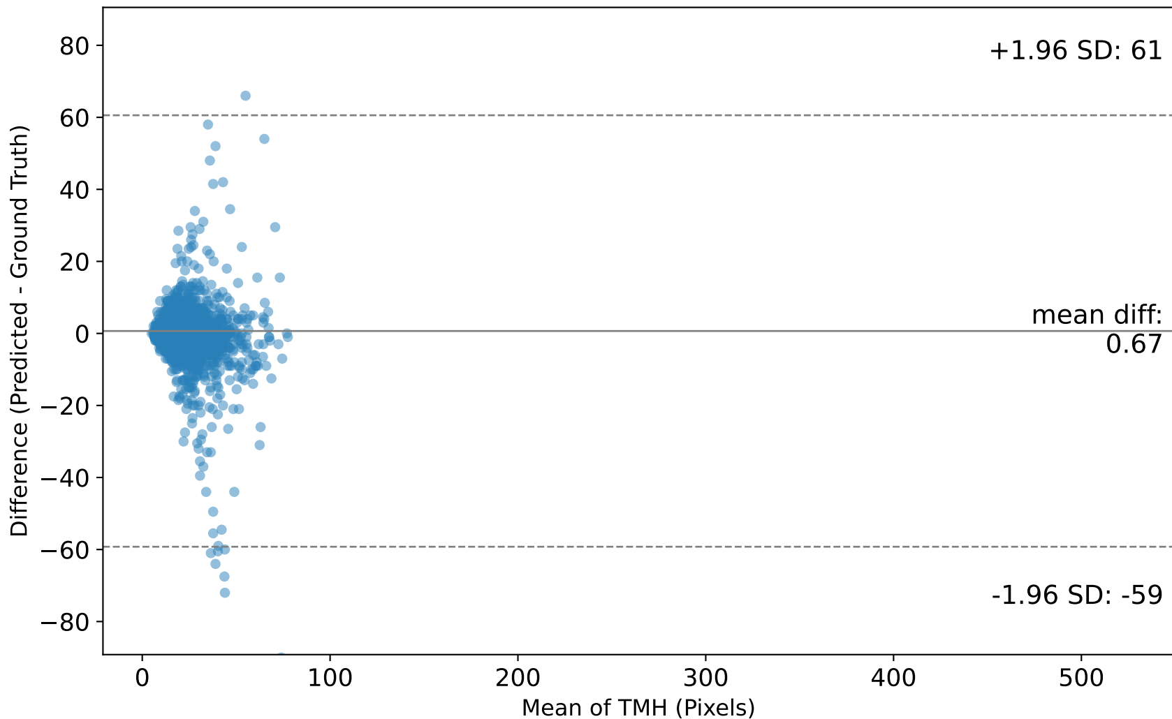
Bland-Altman Plot: ST-SAM vs. Expert Manual Annotation
