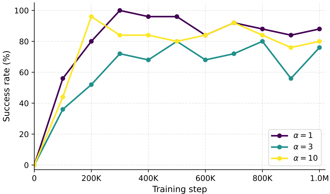
IQL on cube-single: \alpha sweep ( \tau = 0.9 )
