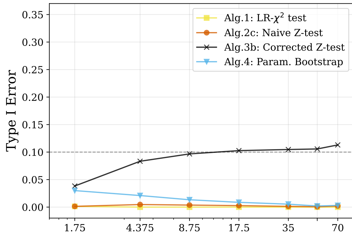
Powerlaw, K = 0.25, \Gamma = 1, n \in [10, 400]
