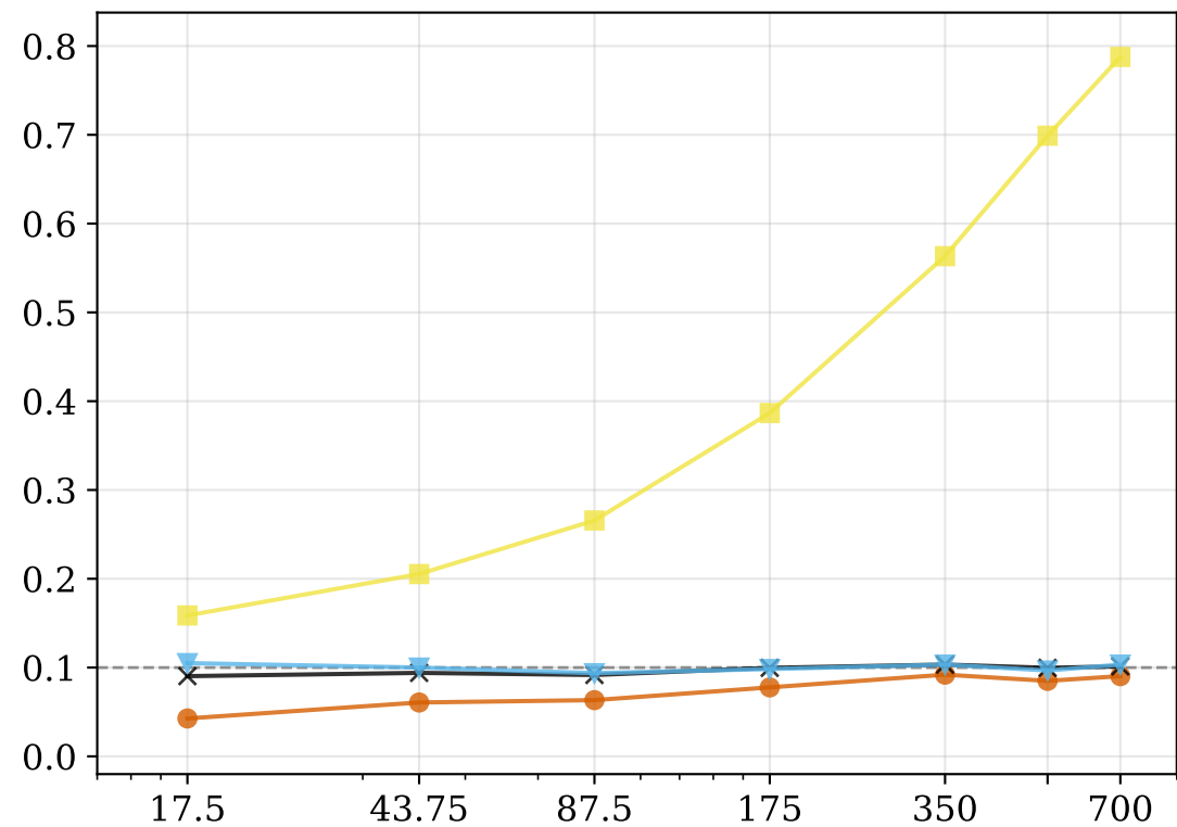
Powerlaw, K = 2.5, \Gamma = 1, n \in [10, 400]
