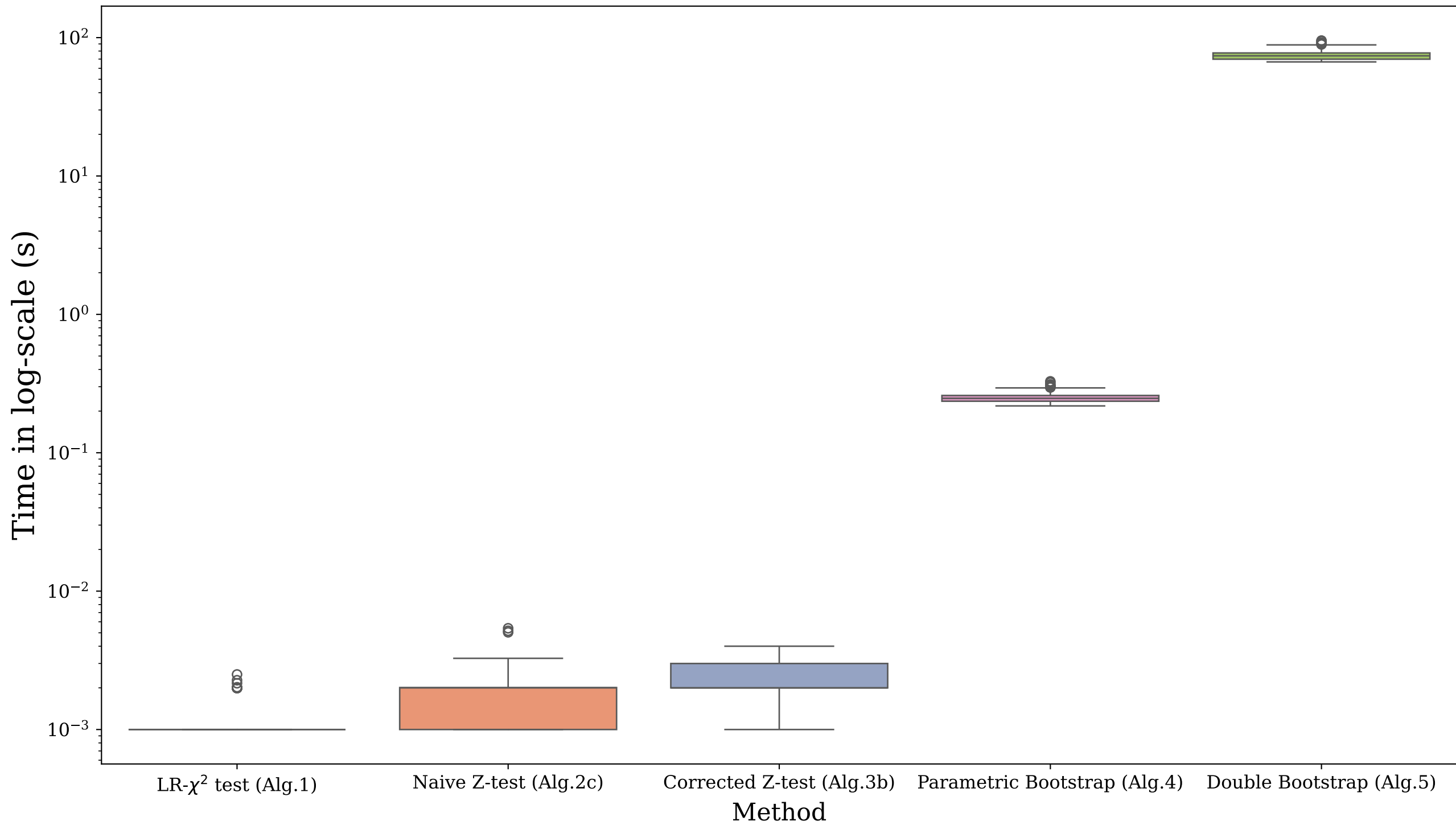
Powerlaw, n = 100 , K = 1 , \Gamma = 1
