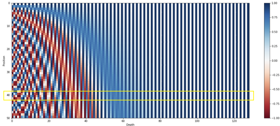
Figure 2 - The 128-dimensional positional encoding for a sentence with the maximum length of 50. Each row represents the embedding vector \vec{v}_i
