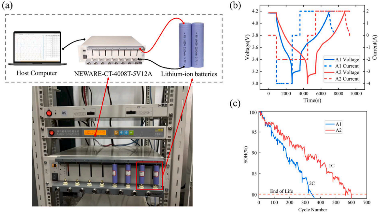
Fig. 2. Full life cycle aging testing of A-series NCM batteries (a) Battery degradation platform in our laboratory for data collection of A1-2 batteries. (b) Charge-discharge protocols of two batteries. Solid lines represent the voltage curves of A1 and A2. Dashed lines represent the current curves of A1 and A2. (c) SOH degradation processes of A1 and A2 with different discharge rate.
