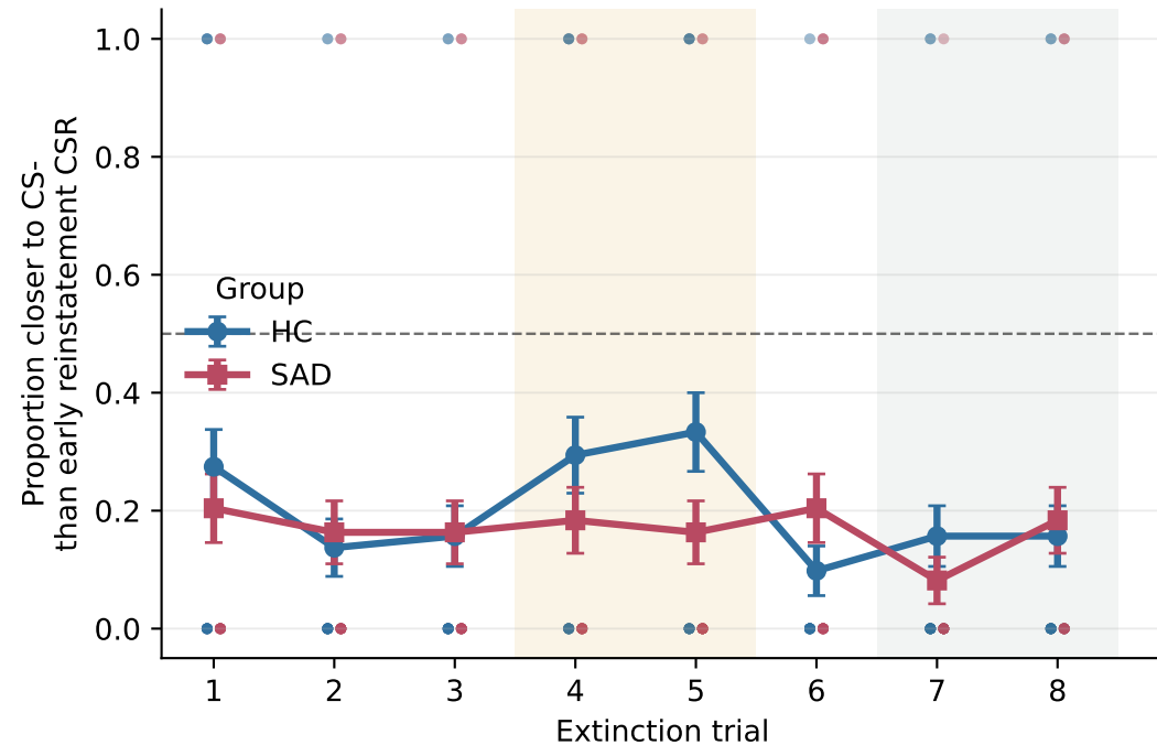
CSS forced-choice CS- evidence
