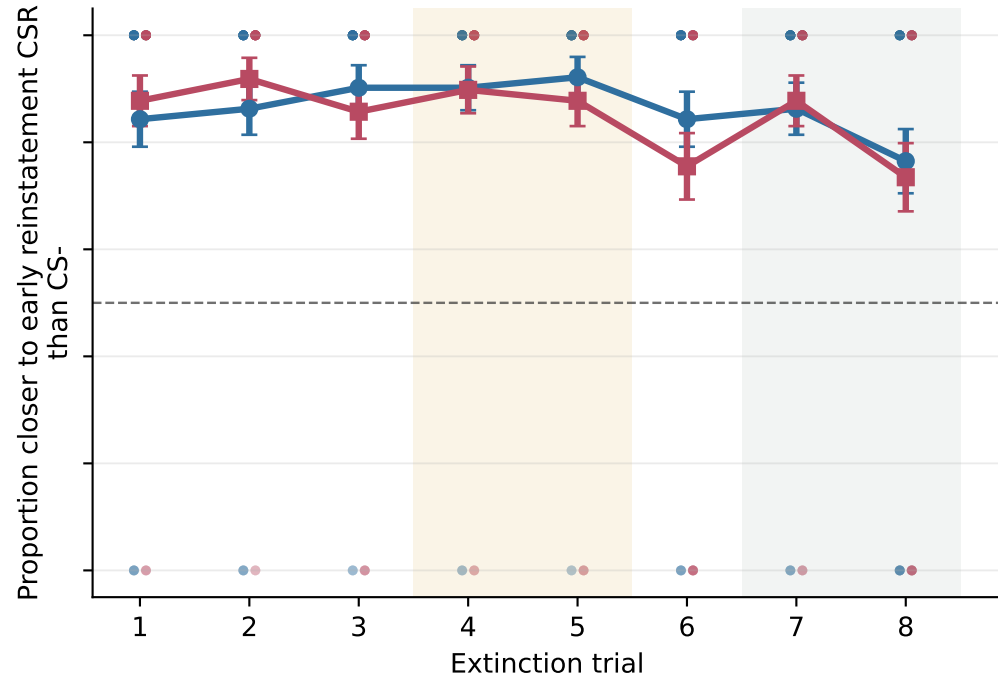
CSR forced-choice early-reinstatement CSR evidence
