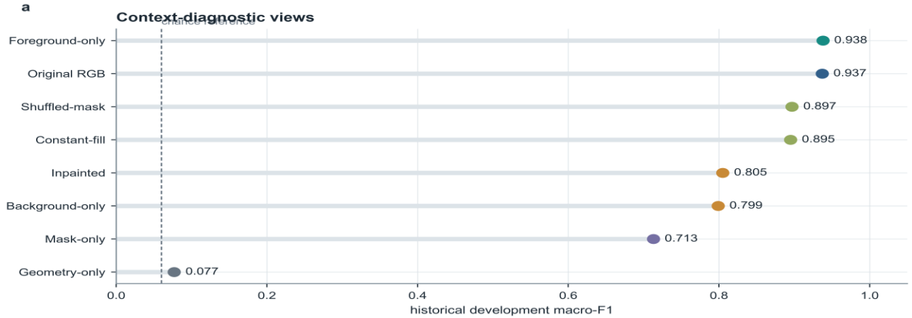
Fig. 3 Context-diagnostic sanity checks on the historical development validation partition. Several views retain substantial predictive non-subject/contextual signal. We reserve the stronger shortcut-susceptibility interpretation for the conflicting-context interventions rather than treating every contextual cue as ecologically spurious.
