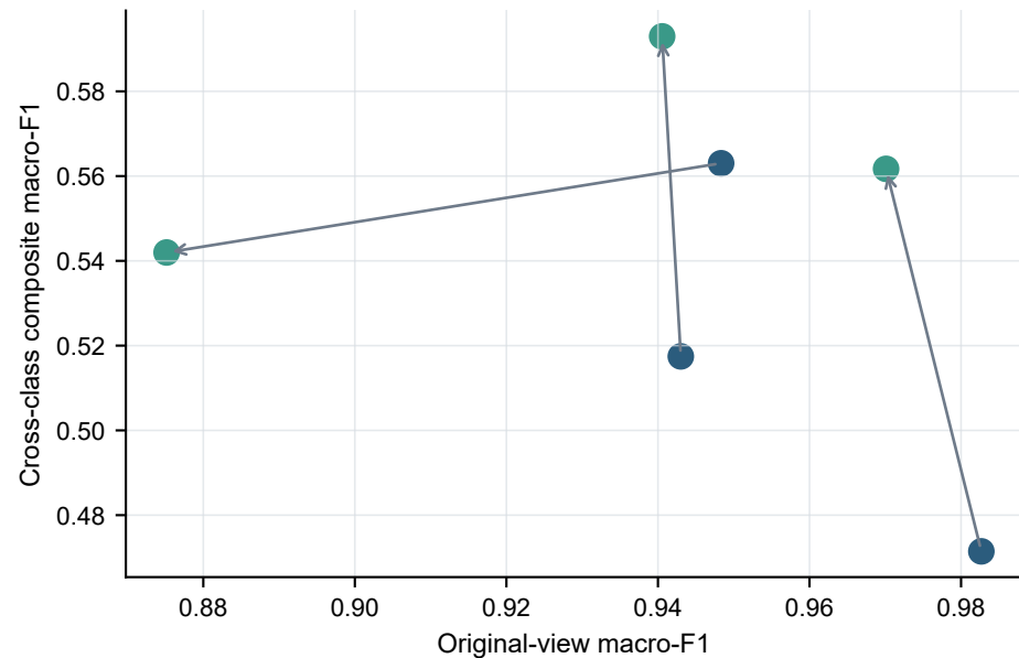
Architecture sensitivity
