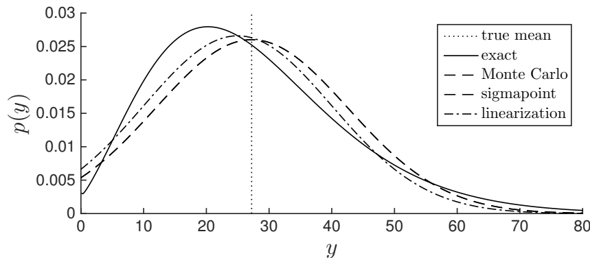
Figure 4.12 Graphical depiction of passing a Gaussian PDF, p(x) = \mathcal{N}(5, (3/2)^2) , through the nonlinearity, y = x^2 , using various methods. We see that the Monte Carlo and sigmapoint methods match the true mean, while linearization does not. We also show the exact transformed PDF, which is not Gaussian and therefore does not have its mean at its mode.
