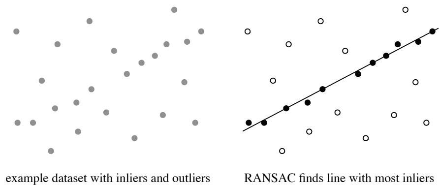
Figure 5.6 Line-fitting example. If a line is fit to all the data, the outliers will have a large impact on the result. The random sample consensus (RANSAC) approach is to classify the data as either an inlier or an outlier and then only use the inliers in the line fit.
