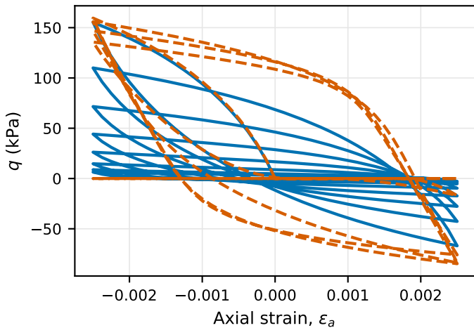
(c) Identical constant-volume cycles
