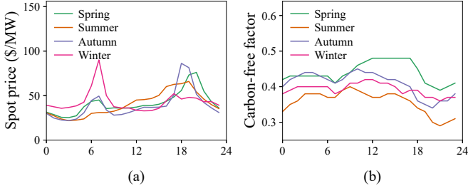
Fig. 1: Hourly spot prices and carbon-free factors for the seasonal representative days. (a) Spot price. (b) Carbon-free factor.
