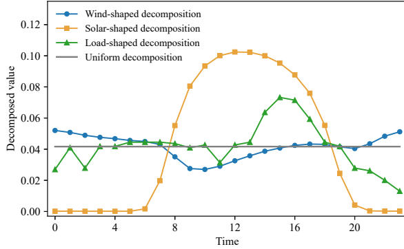
Fig. 2: Normalized hourly delivery profiles of the four contract shaping conventions.
