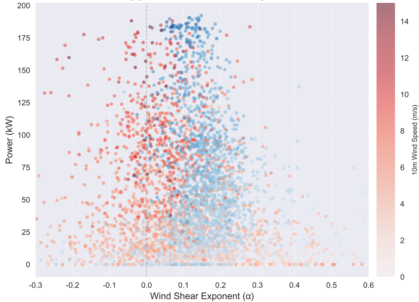
(C) Wind Shear vs Power Output
