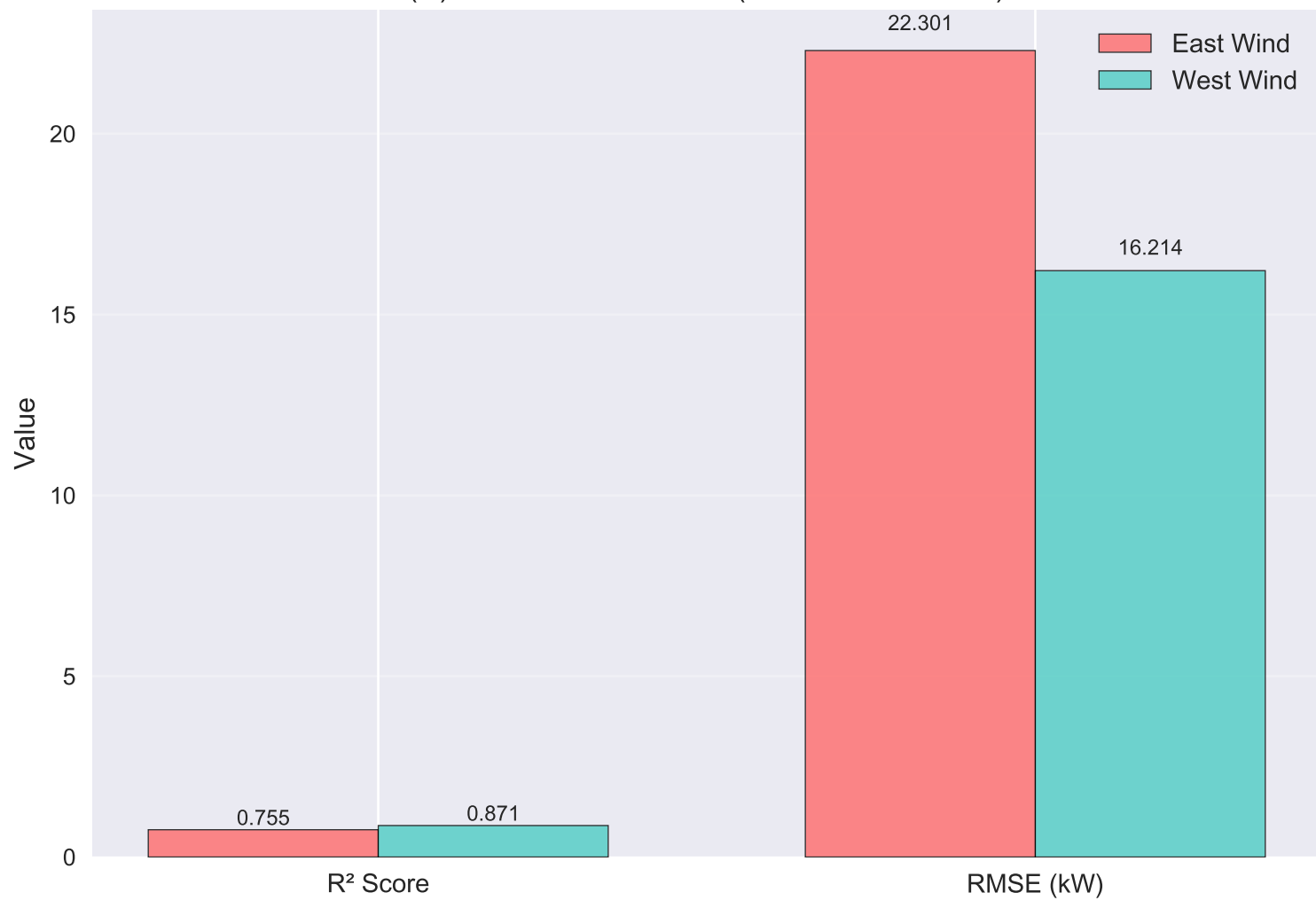
(D) Model Performance (with Wind Shear \alpha )
