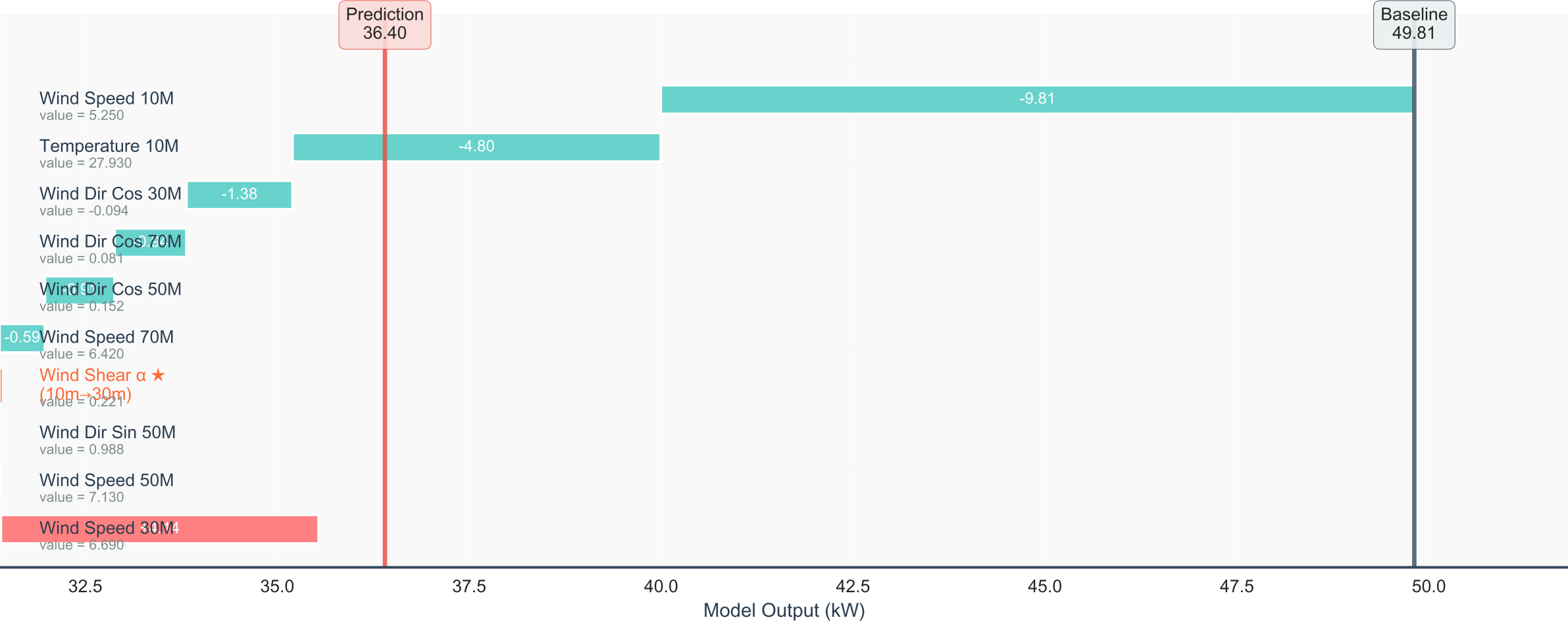
(C) Feature Contributions for Single Prediction (36.4 kW)
