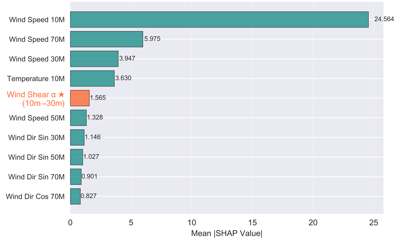
(A) Feature Importance
