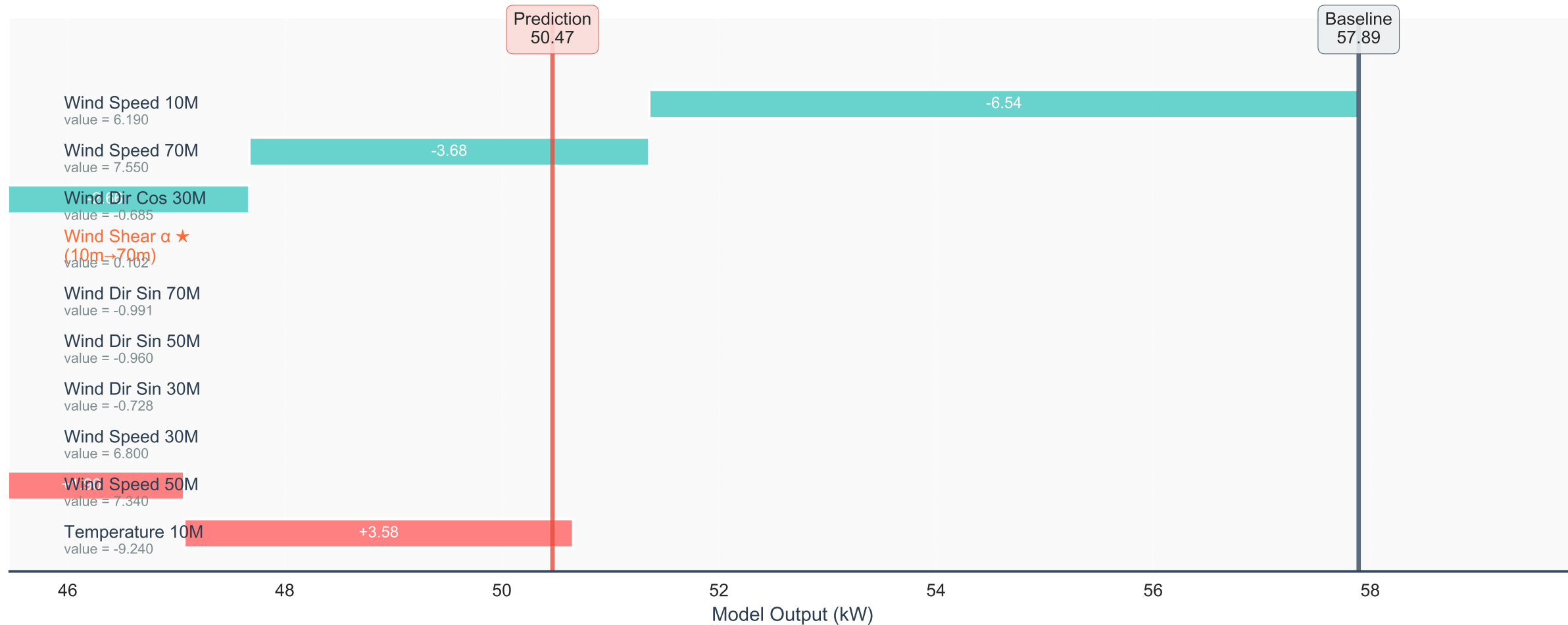
(C) Feature Contributions for Single Prediction (50.5 kW)
