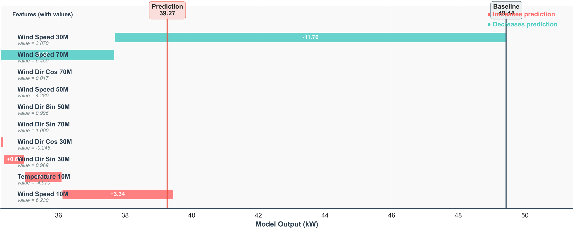
(C) Feature Contributions for Single Prediction (39.3 kW)
