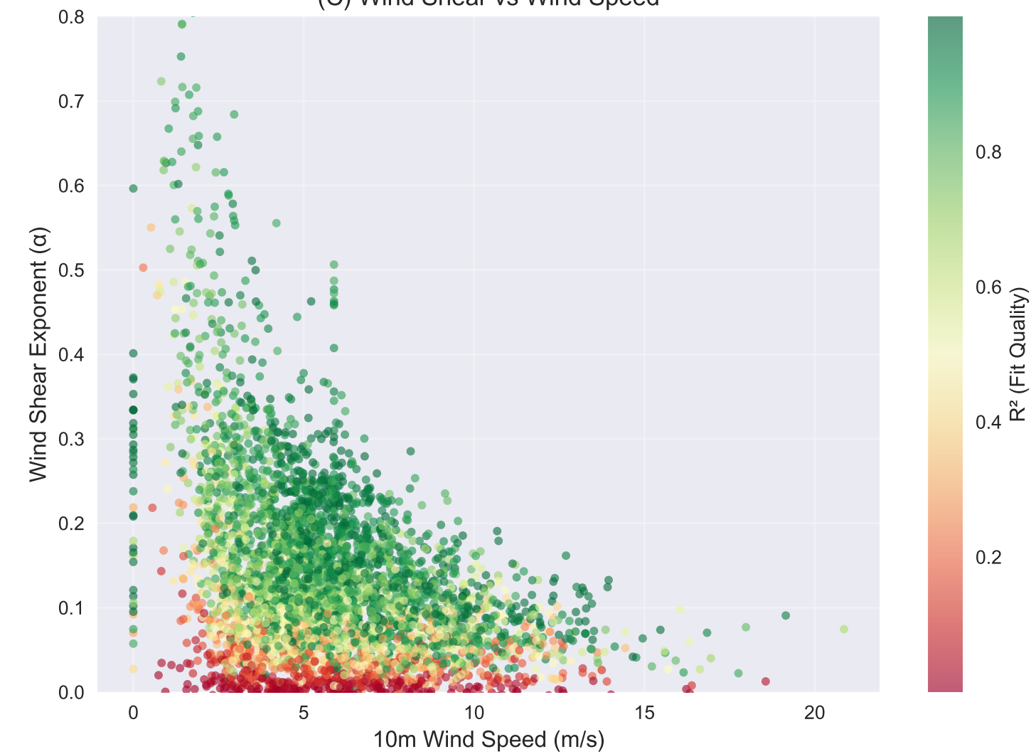
(C) Wind Shear vs Wind Speed
