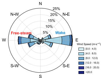
A Wind Rose at Hub Height
