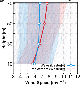
D Free-stream vs. Wake Regime
