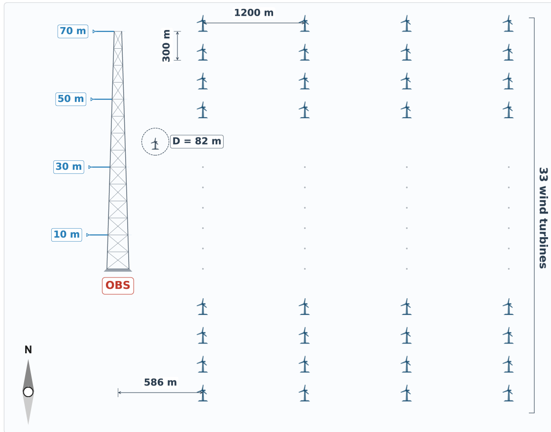
Figure S1. Schematic of the wind farm layout and meteorological mast configuration. The 70-m observation mast (OBS) is located 586 m west of the first turbine column. Wind speed and direction are measured at four heights (10 m, 30 m, 50 m, and 70 m). The farm comprises 134 turbines (33 rows \times 4 columns, plus 2 additional turbines) with approximately 300-m row spacing and 1200-m column spacing. Each turbine has a rotor diameter ( D ) of 82 m and a hub height of 61.5 m. Westerly winds (from left) represent free-stream conditions at the mast, whereas easterly winds (from right) traverse the turbine array before reaching the mast, corresponding to wake-influenced conditions.
