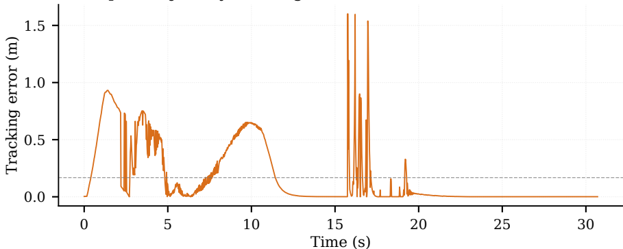
(b) Tip-to-trajectory tracking error
