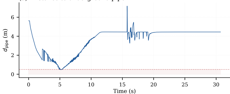
(a) Distance to underground pipe
