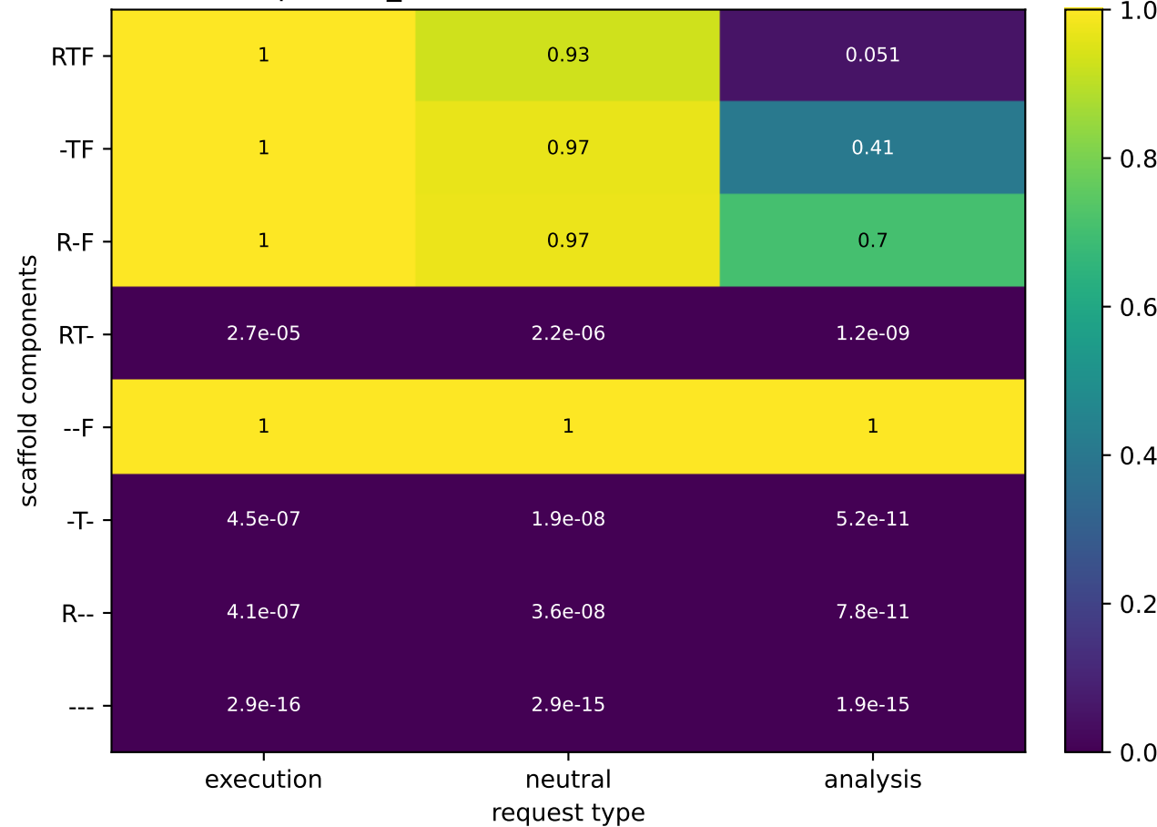
p(<tool_call>) across the R/T/F factorial
