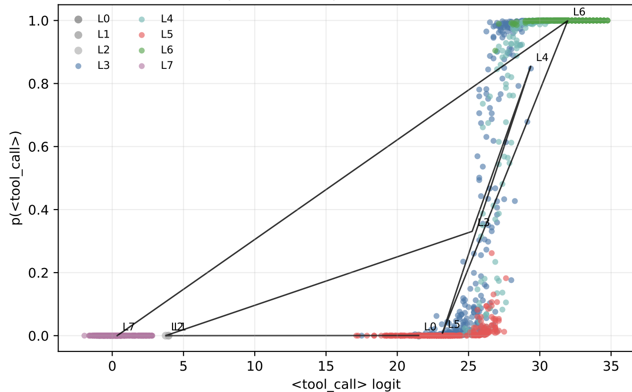
Request ladder: point-level behavior
