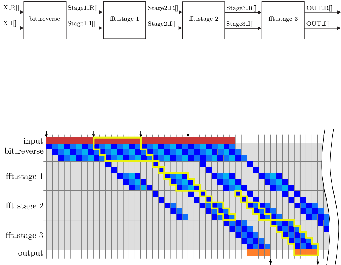
Figure 5.8: Dividing the FFT into different stages allows for task pipelining across each stage. The figure shows an example with three FFT stages (i.e., an 8 point FFT). The figure shows four 8-point FFT executing simultaneously.
