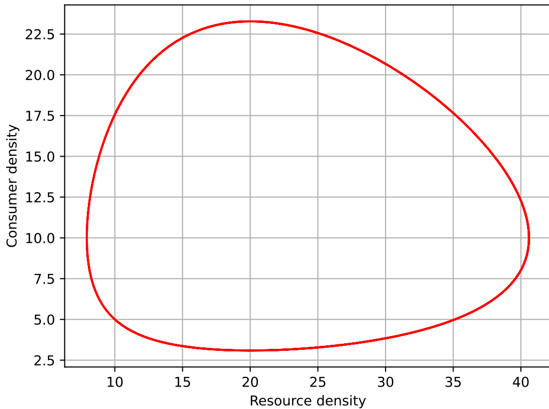
Lotka-Volterra Phase Plot (C vs R)
