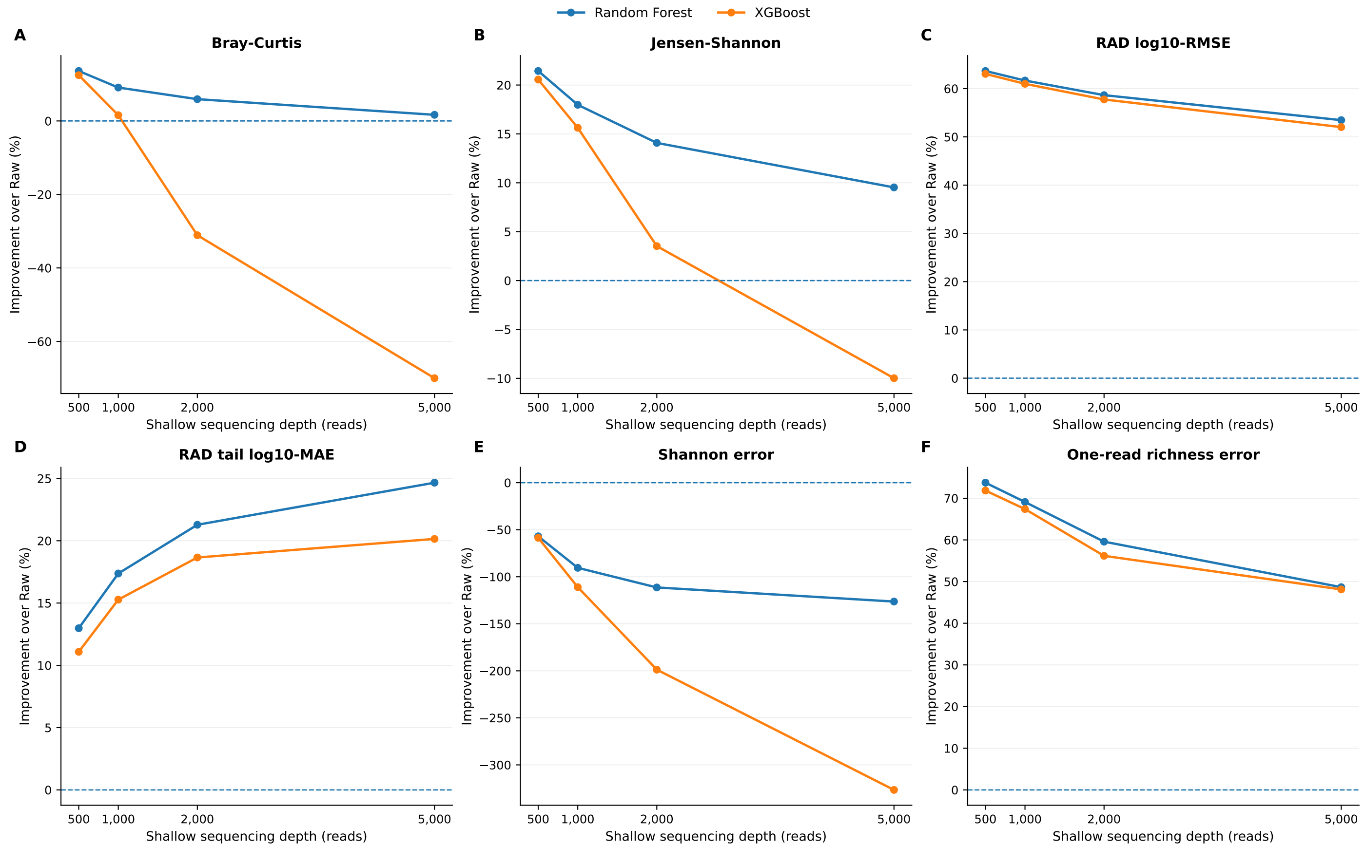
Figure 11. Model improvement over Raw shallow RA across depths
