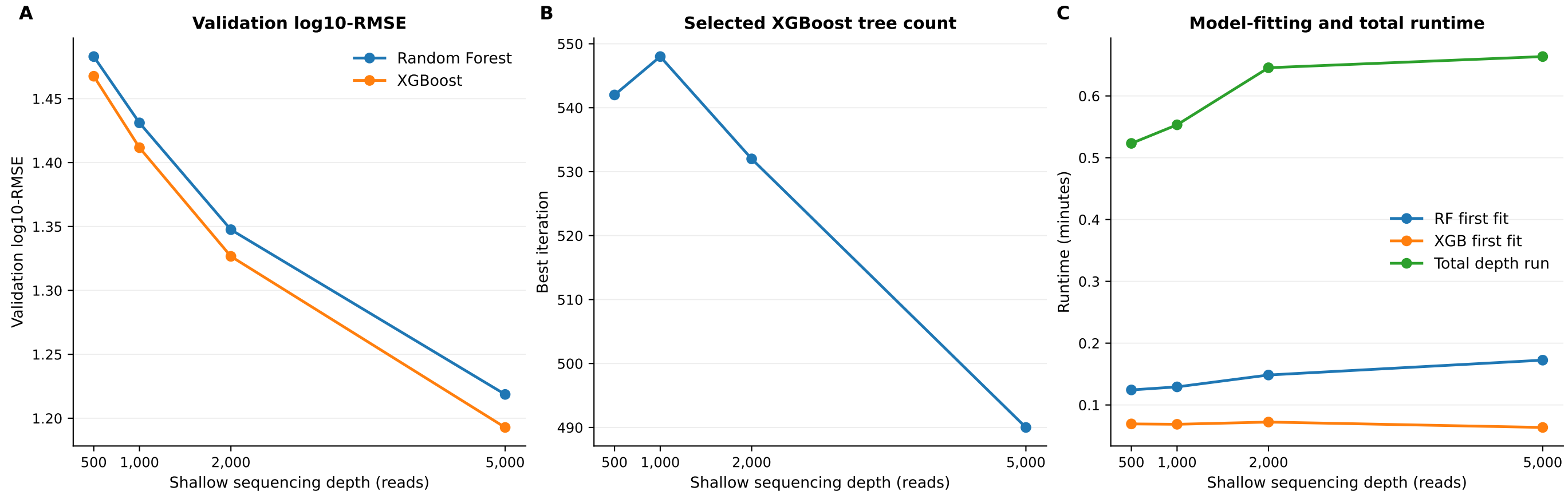
Figure 14. Validation performance and depth-specific model selection
