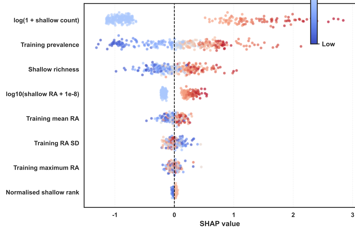
XGBoost: SHAP distribution
