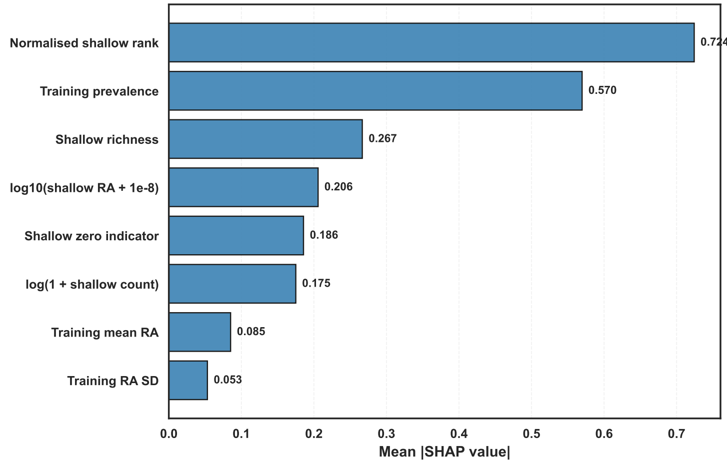
XGBoost: global importance
