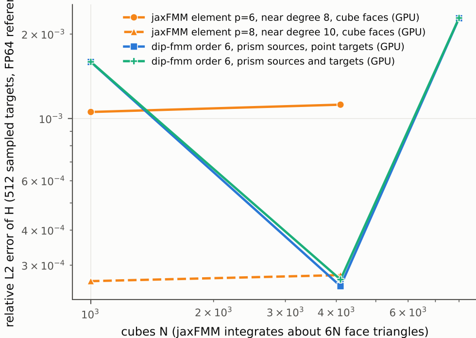
Uniformly magnetised touching cubes, targets at cube centres: achieved accuracy [interim-74-of-241]
