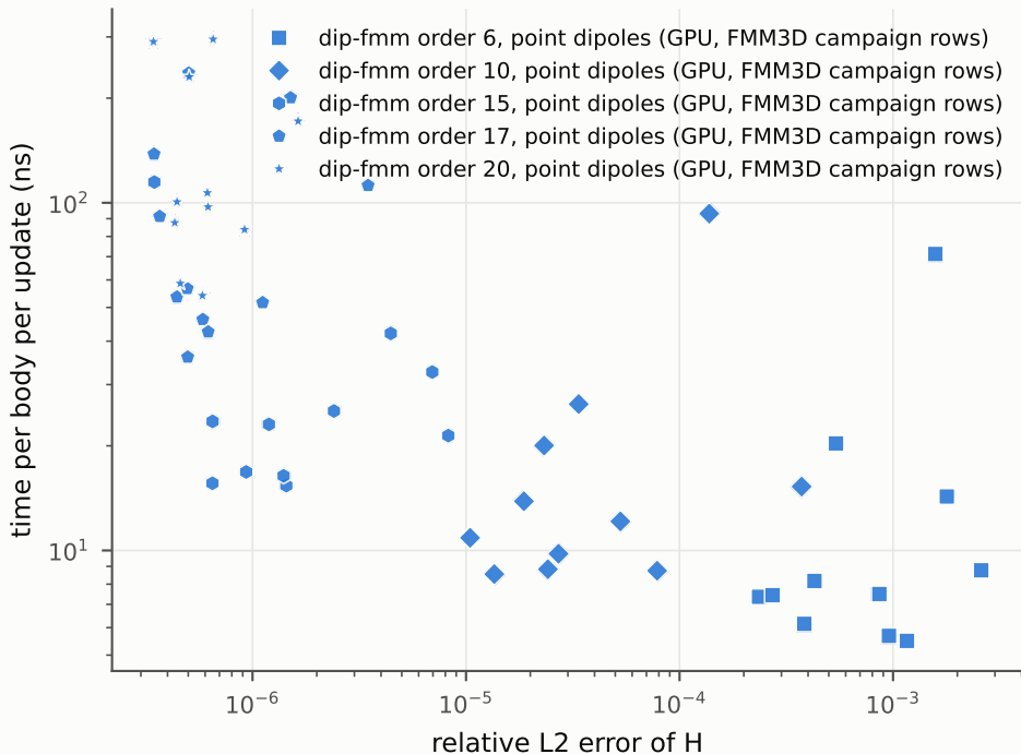
Point dipoles at lattice sites, identical point targets: throughput at achieved accuracy (one marker per N, point targets) [interim-74-of-241]
