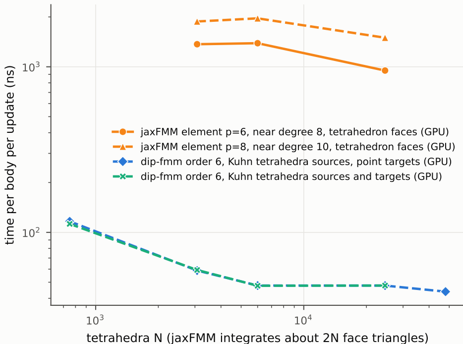
Uniformly magnetised Kuhn tetrahedra, targets at centroids: throughput, host to host [interim-74-of-241]
