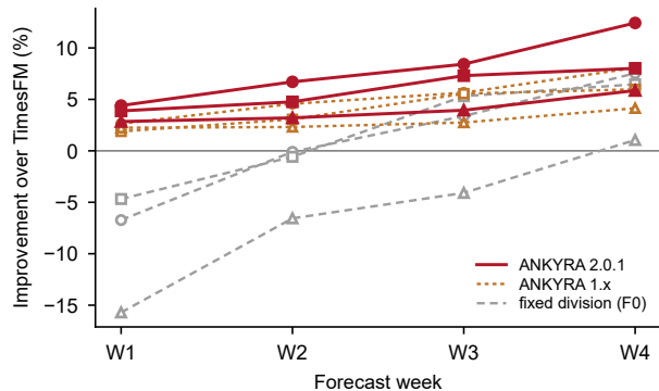
c Lead-week profile vs TimesFM
