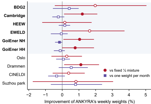
b Weekly per-unit weights against simpler mixing
