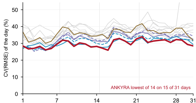
a HKUST campus: hourly error of each forecast day
