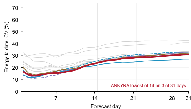
d Helsinki city buildings: error of the energy delivered to date
