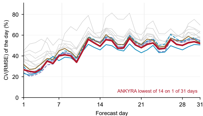
c Helsinki city buildings: hourly error of each forecast day
