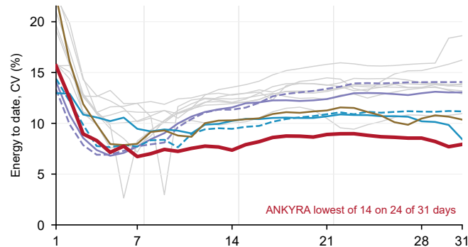
b HKUST campus: error of the energy delivered to date
