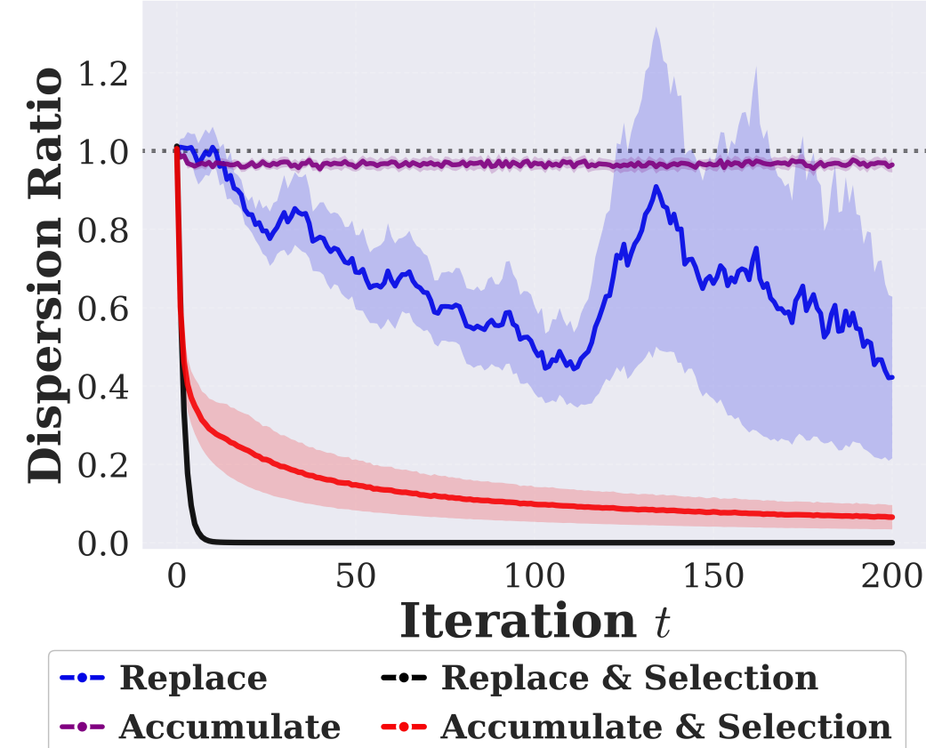
Laplace
