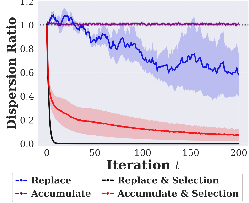
Gaussian mixture
