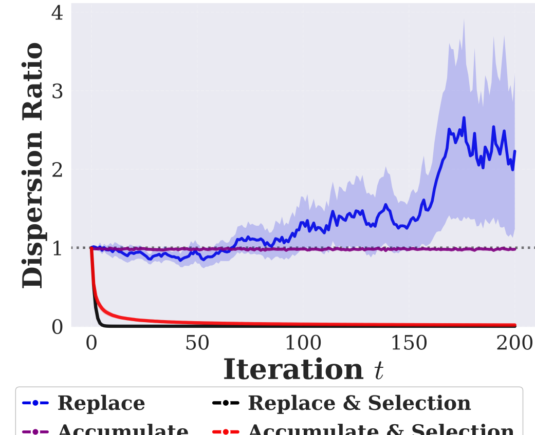
Laplace
