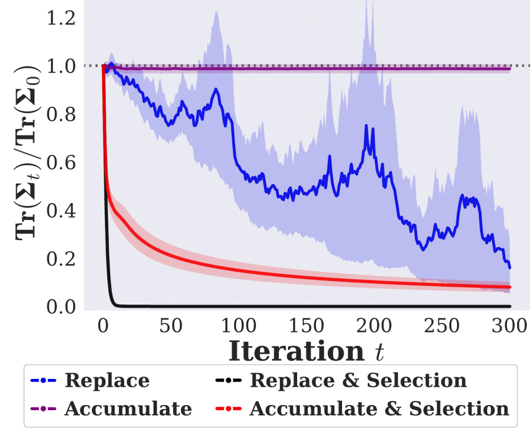
Gaussian mixture
