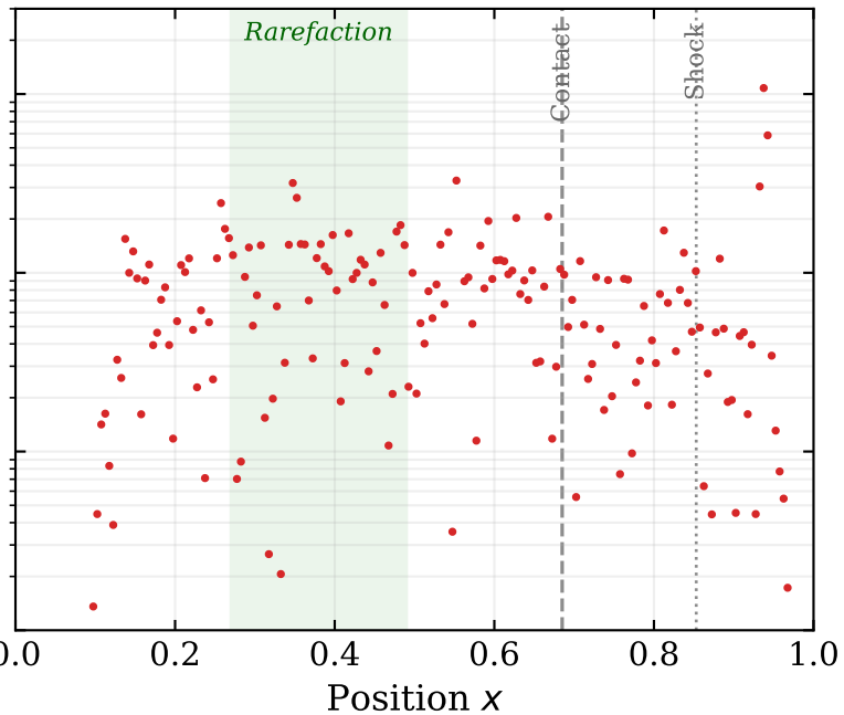
(b) HLL
