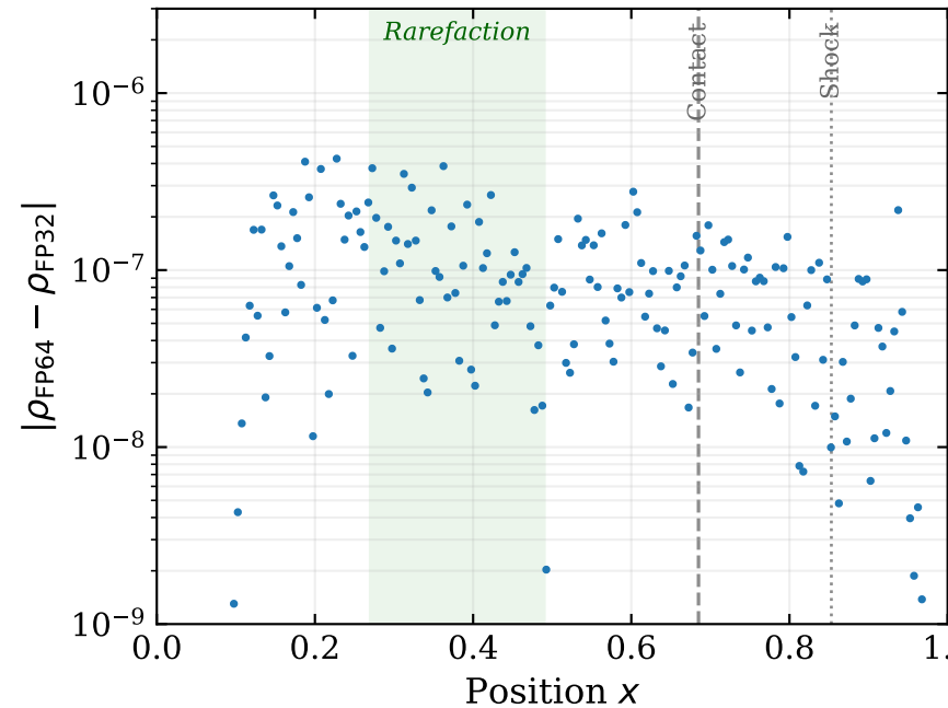
(a) HLLC
