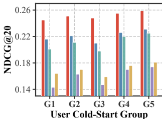
(a) Performance w.r.t. cold-start user groups
