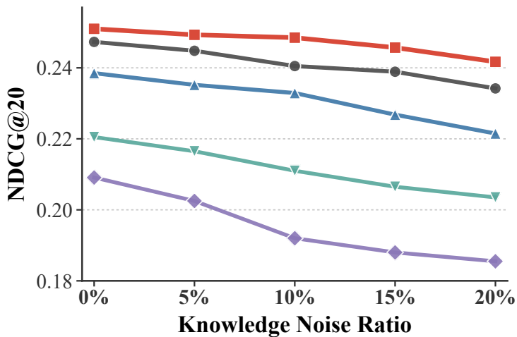
(b) Last-FM
