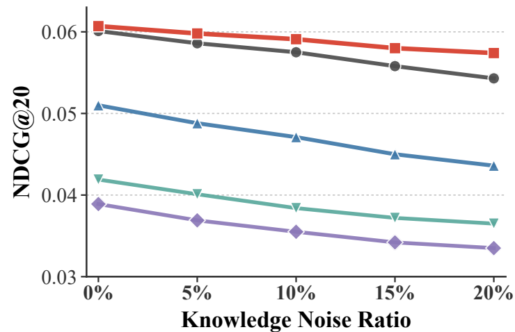
(a) MIND
