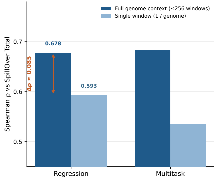
a Sequence-level performance
