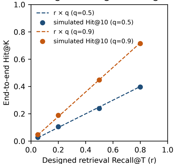
A Hit@K = Recall@T × oracle@K
