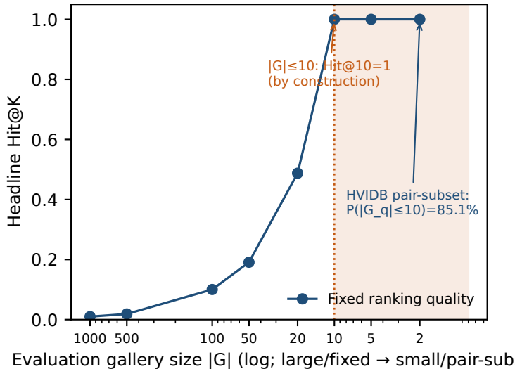
B Hit@K vs gallery size (fixed scores)
