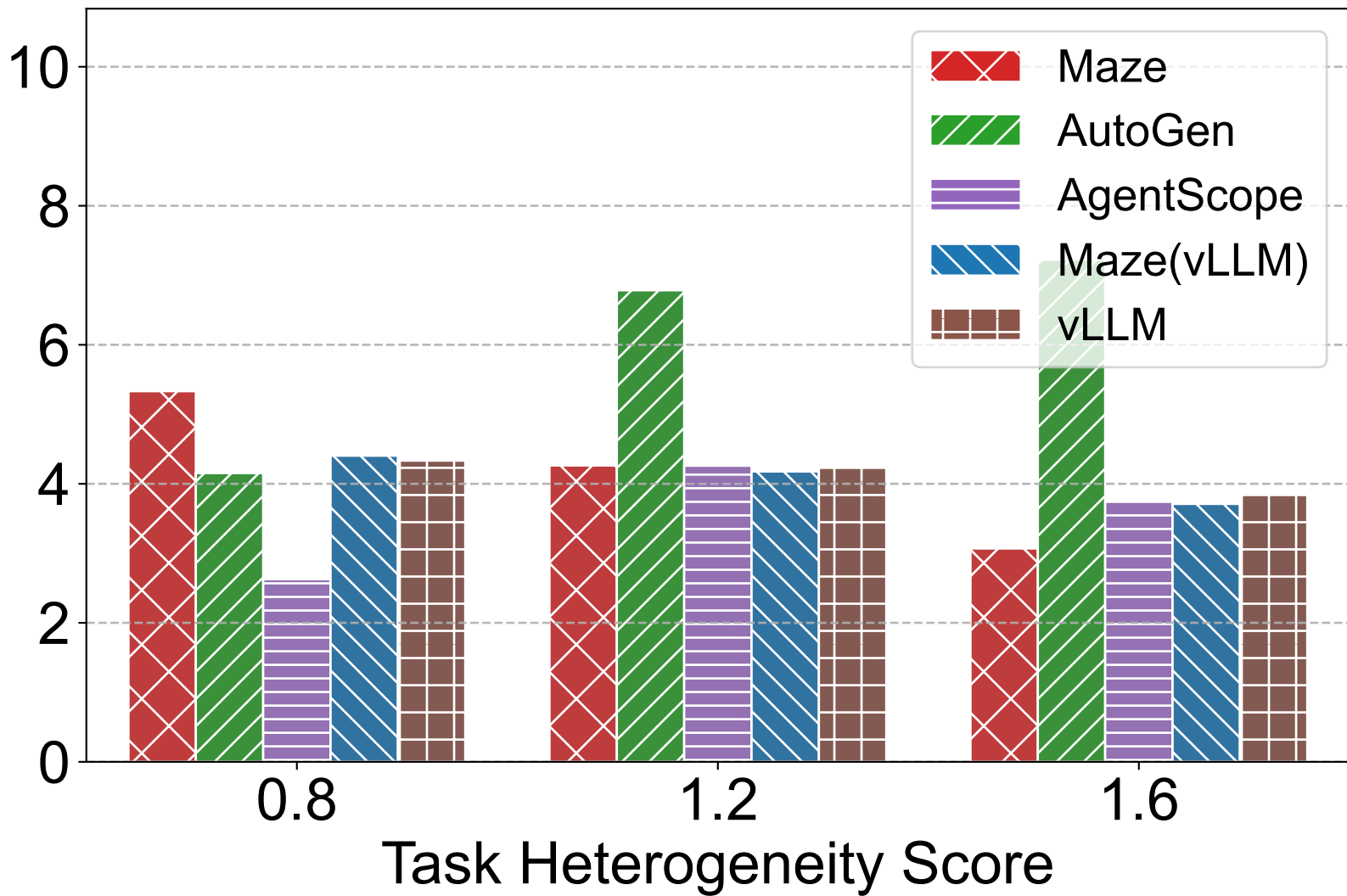
CPU Utilization (%)
