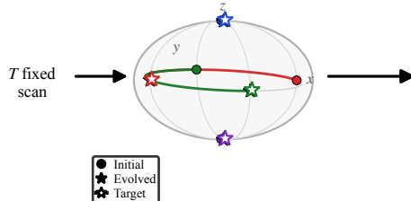
(b) Propagator
