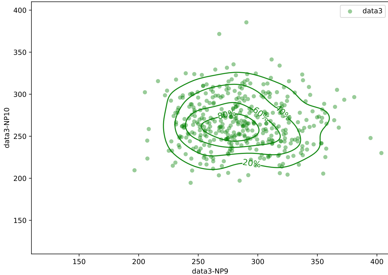
KDE contour for data3 heat flux
