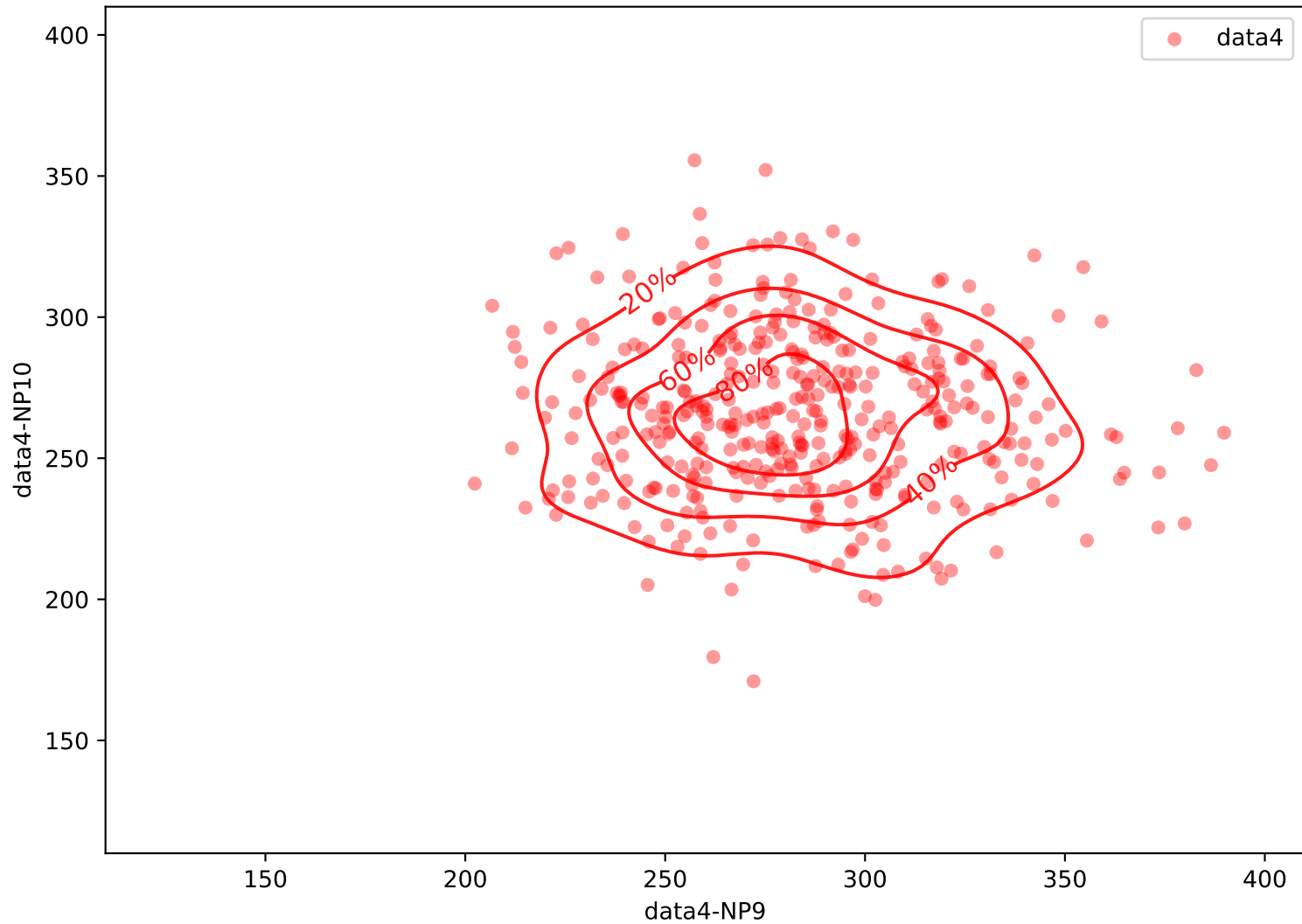
KDE contour for data4 heat flux
